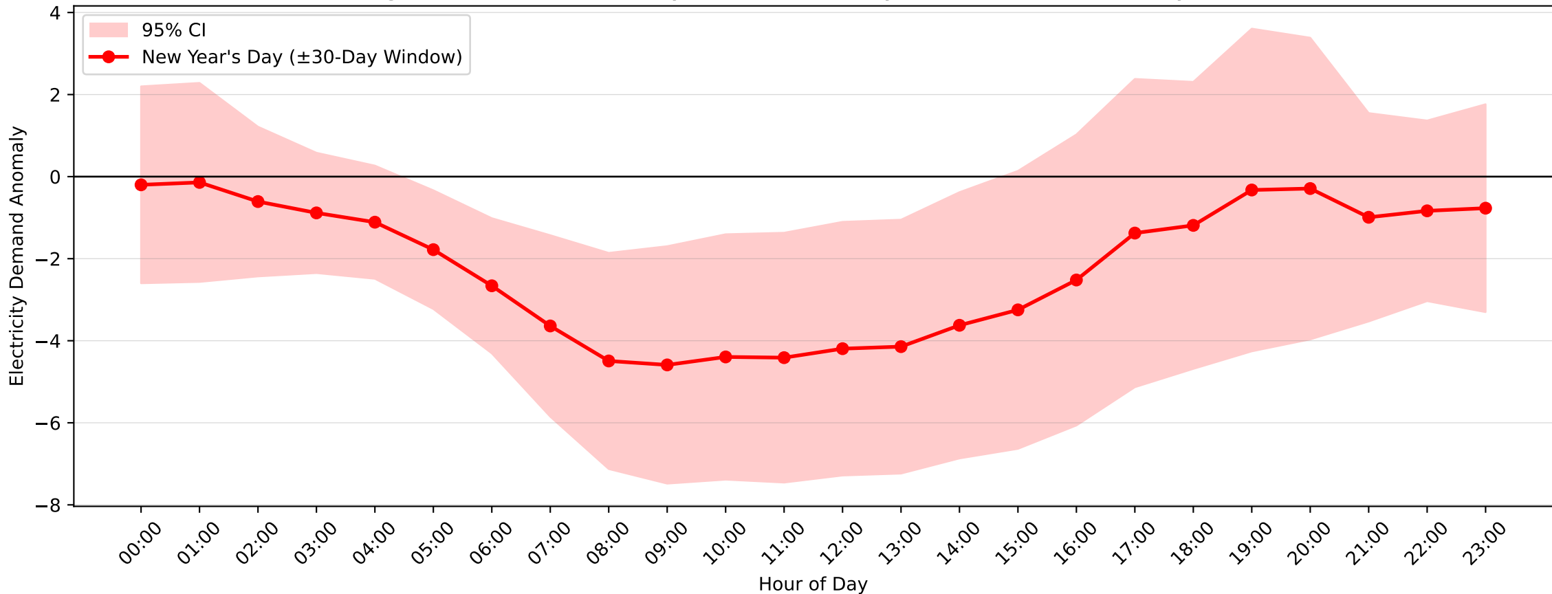
Caringbah Demand Anomaly: New Year's Day (2004–2017, \pm 30 -Day Window)
